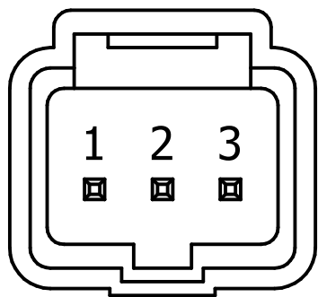
Power supply plug 03T-JWPF-VSLE-S (male)
