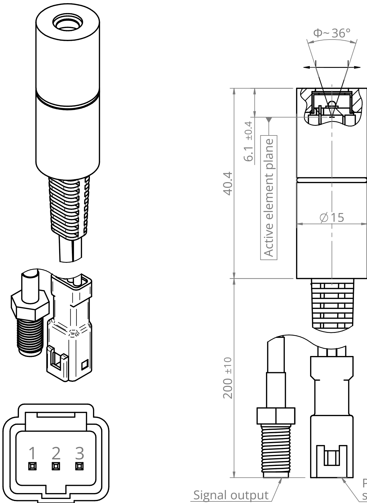
Power supply plug JST 03T-JWPF-VSLE-S (male)
