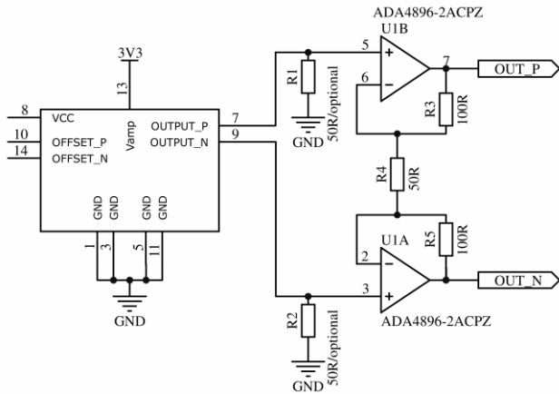
FIGURE 7. Example differential voltage amplifier with gain=5 and DC coupling. R1/R2 are not required for slowly changing signals
