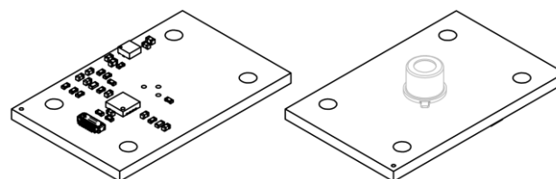
FIGURE 1. The TO46-3.6k-AMS amplifier (detector is not included)
