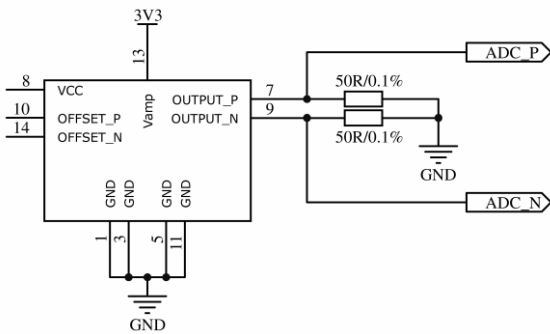
FIGURE 5. Outputs termination for high-speed signals
