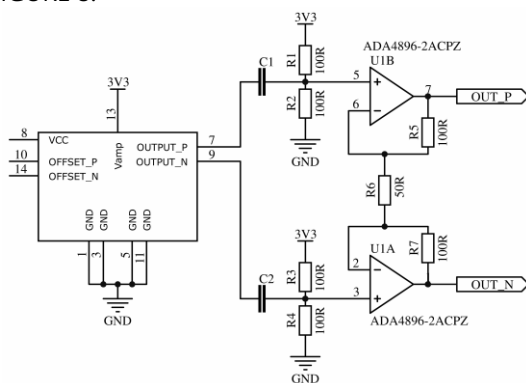
FIGURE 8. Example differential voltage amplifier with gain = 5 and AC coupling
