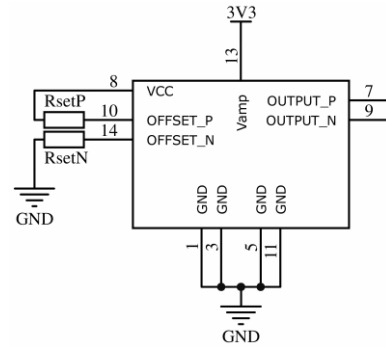
FIGURE 6. Adjusting differential offset of outputs using two resistors. R_{setP} and R_{setN} can be set to 0 \Omega for maximum available offset
