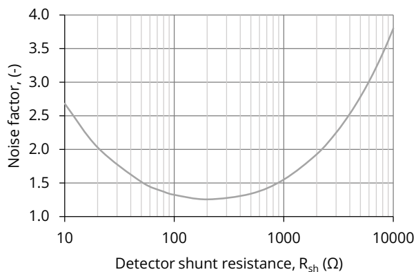
FIGURE 4. Noise factor vs Detector shunt resistance of the detector at 1 kHz
