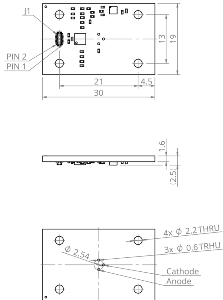
FIGURE 9. Dimensions of the TO46-3.6k-AMS amplifier (given in mm)
