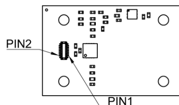
FIGURE 3. Pins ordering on the J1 connector
