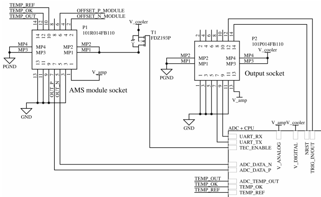
FIGURE 1. Schematic diagram of the AMS-DIG-PROC. All unused pins of P2 should be left floating.
