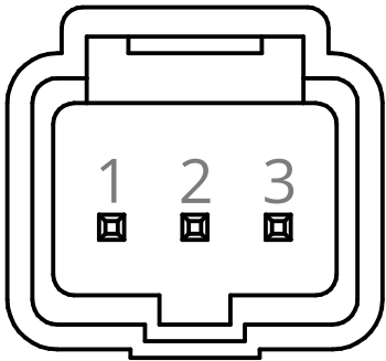
Power supply plug JST 03T-JWPF-VSLE-S (male)
